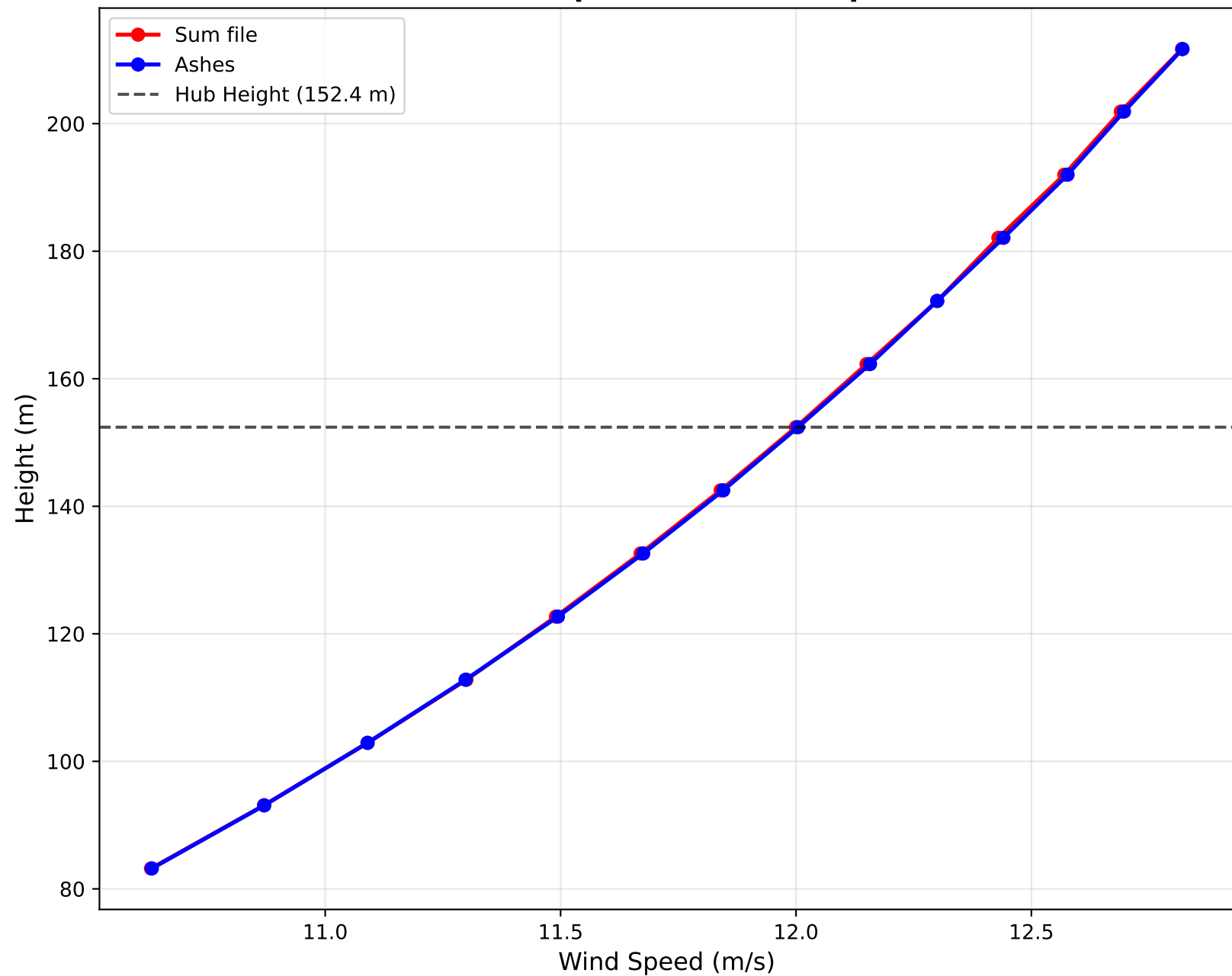
Mean Wind Speed Profile Comparison
